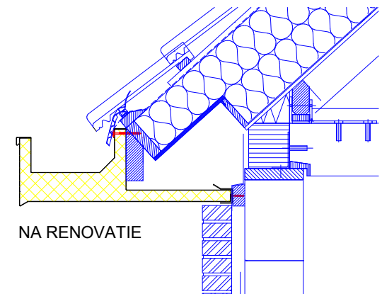
Renovation detail
