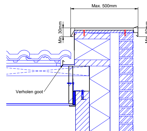
Capping detail
