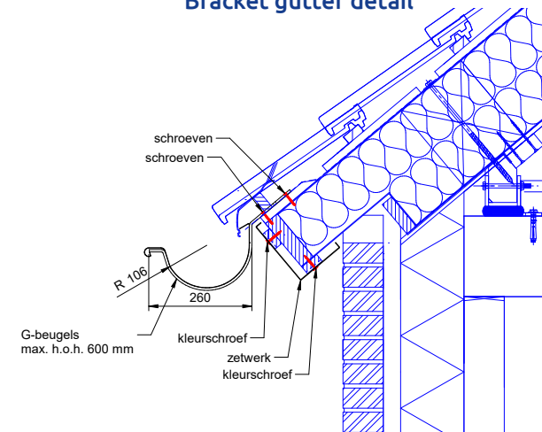
Bracket gutter detail
