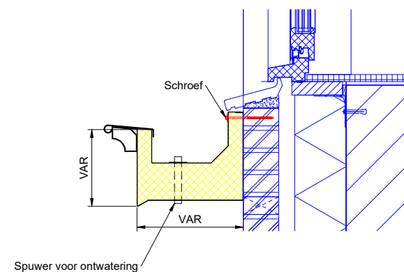
Planter detail
