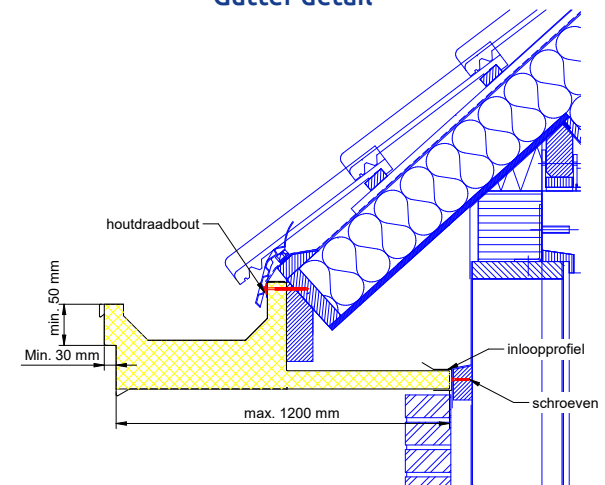
Gutter detail
