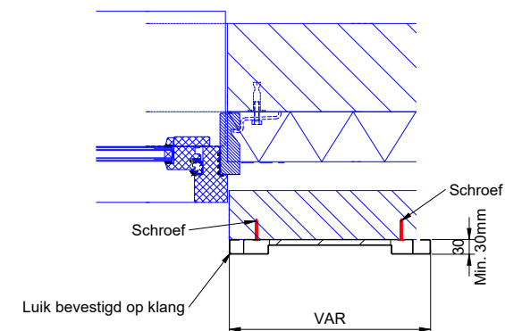
Shutter detail
